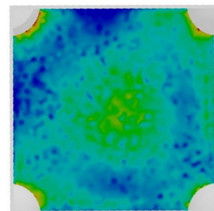
Fig. 5. Equivalent stress distribution of cover.
