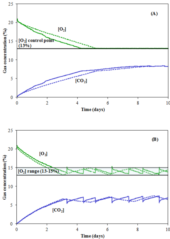
Fig. 1. Comparison between passive diffusion tube and active flushing systems adopted to green pepper container, which was subjected to control at (A) a set O 2 concentration of 13% and (B) a set range of O 2 concentration of 13~15% at 10°C. Solid lines are for active flushing system while dashed lines are for passive diffusion tube system.
