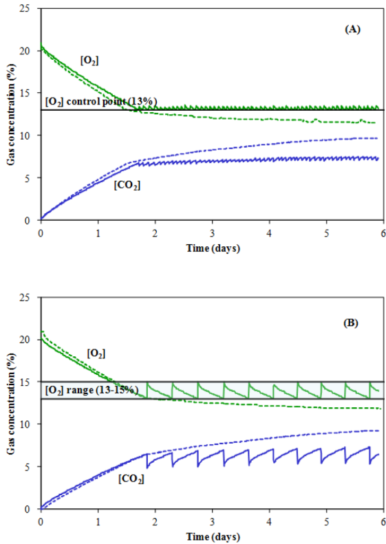
Fig. 2. Gas concentration in green pepper container applied to (A) one point control of 13% O 2 and (B) range control of 13~15% O 2 at 20°C. Solid lines are for active flushing system while dashed lines are for passive diffusion tube system.
