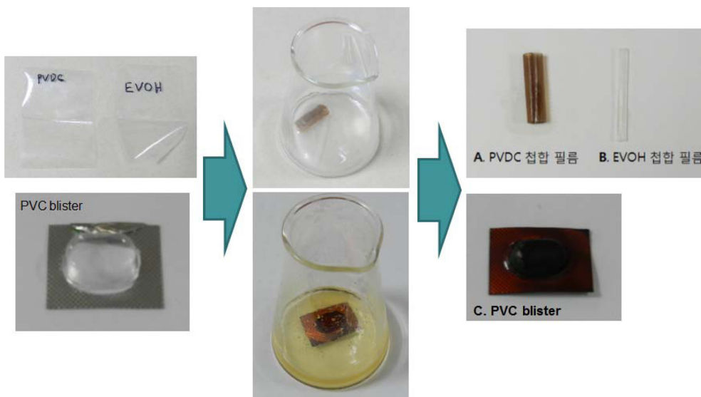
Fig. 2. Brief experimental Results of specimen immersed in the reagent solution to verify the performance of the prepared reagent solution: (A) PVDC laminated film; (B) EVOH laminated film; (C) PVC blister.
