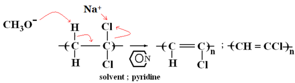
Fig. 1. Chemical reaction of reagent solution with Cl included packaging materials.
