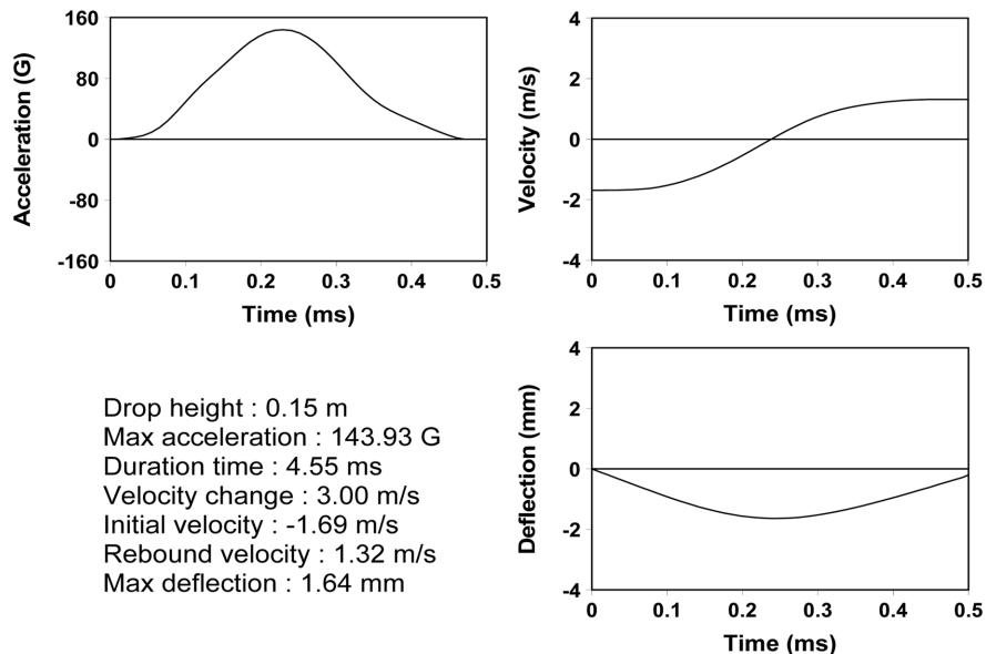
Fig. 3. Acceleration, velocity and deflection in an impact for the single wall corrugated fiberboard.
