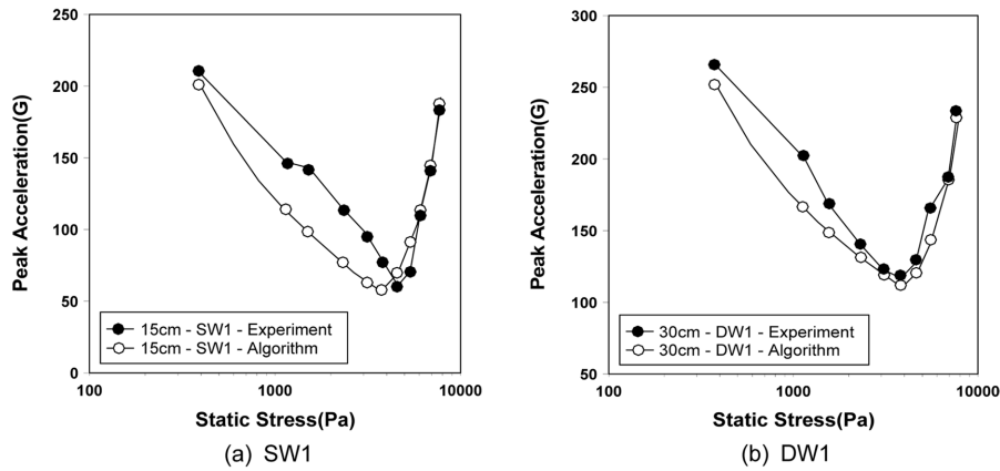
Fig. 7. Peak acceleration-static stress curve of the corrugated fiberboard.
