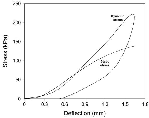
Fig. 4. Dynamic and static stress behaviors for the single wall corrugated fiberboard.
