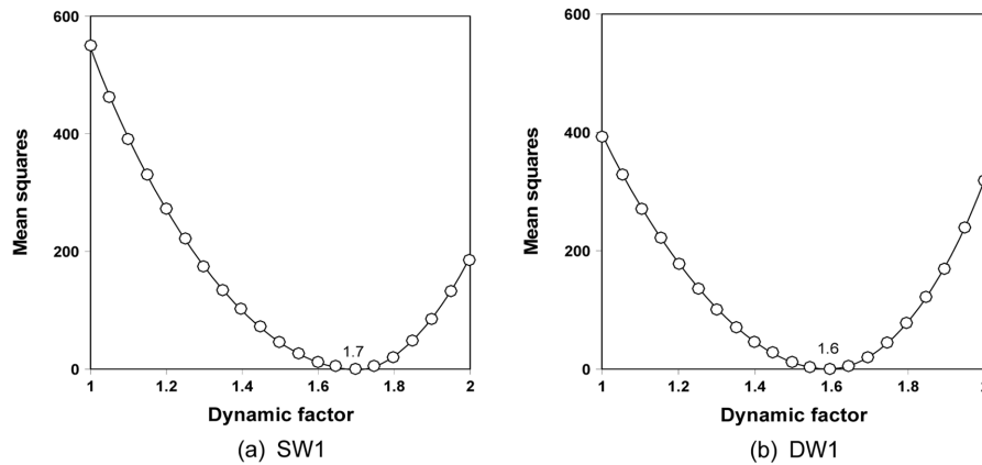
Fig. 6. Dynamic factor using the developed algorithm.
